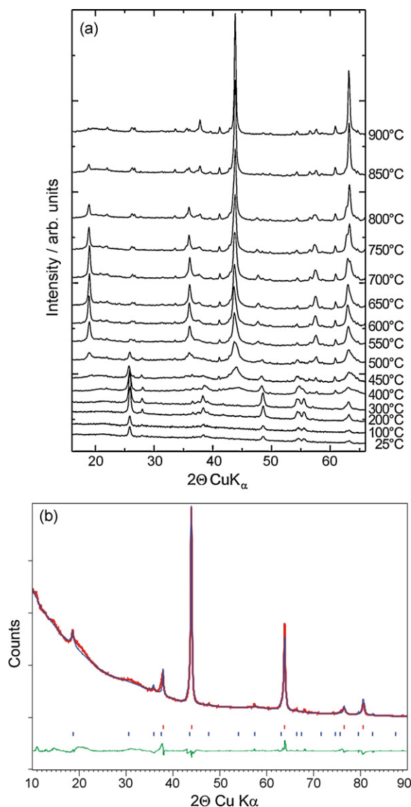
Fig. 1. (a) Evolution of the structure during the heating of initial precursor mixture as measured with an in situ high-temperature XRD. (b) Refinement for the XRD pattern obtained from LVT850 sample.
