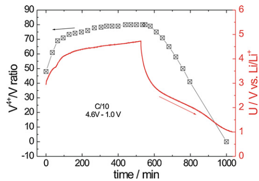
Fig. 6. The relative amount of \text{V}^{4+} component in the \text{Li}_{2-x}\text{VTiO}_4 positive material during the first cycle of charge/discharge process, determined from V XANES spectra (left axis) and corresponding electrochemical curve obtained during in situ measurement (right axis).
