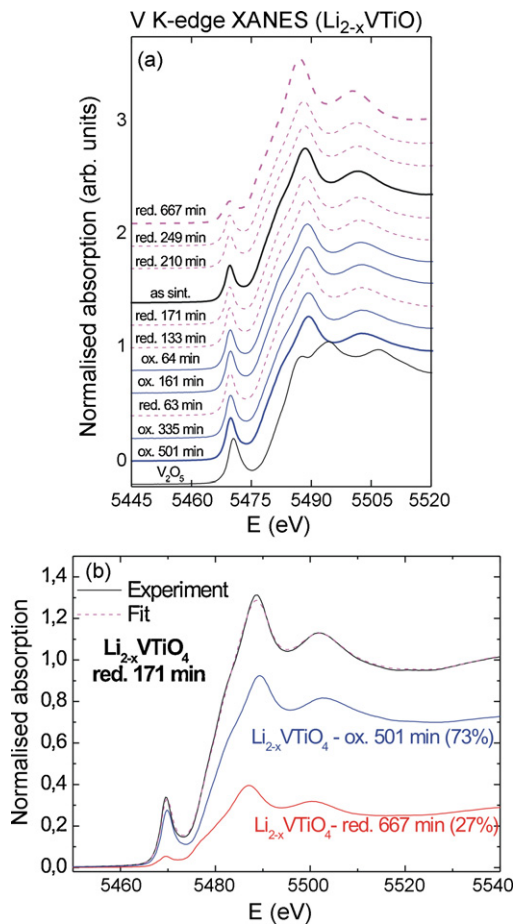
Fig. 5. (a) The V K-edge XANES spectra of \text{Li}_{2-x}\text{VTiO}_4 sample during the oxidation and reduction, and \text{V}_2\text{O}_5 reference compound. The spectra are displaced vertically for clarity. (b) V K-edge XANES spectrum of \text{Li}_{2-x}\text{VTiO}_4 sample after 171 min of reduction: Solid line—experiment; magenta dashed line—best-fit linear combination of XANES profiles of \text{Li}_2\text{VTiO}_4 sample after 667 min of reduction ( \text{V}^{3.0+} ) and after 501 min of oxidation ( \text{V}^{3.8+} ) (both components are shown below). (For interpretation of the references to color in this figure legend, the reader is referred to the web version of the article.)
