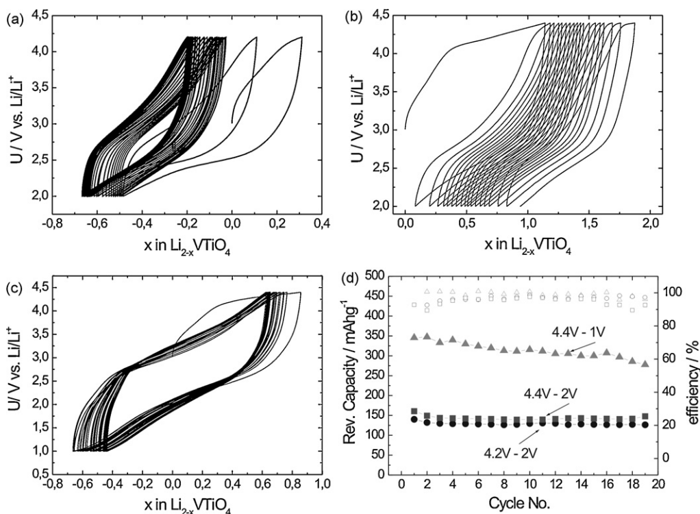
Fig. 3. (a–c) Cycling behaviour of LVT850 sample in the three different electrochemical windows obtained with C/10 cycling rate at room temperature: between 2 V and 4.2 V (a), between 2 V and 4.4 V (b), and between 1 V and 4.4 V (c). Cycling performance of LVT850 sample cycled within three different voltage windows (reversible capacity—filled symbols and cycling efficiency—open symbols) (d).
