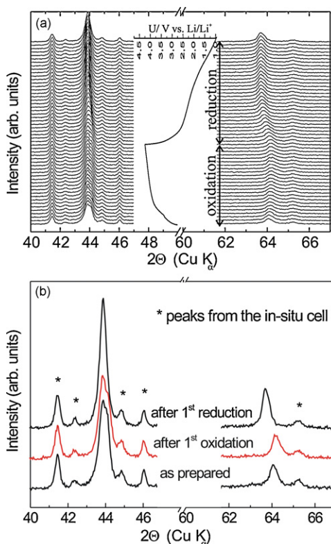
Fig. 4. Voltage limited in situ X-ray diffraction experiment on LVT850 sample: (a) obtained X-ray diffraction patterns during oxidation/reduction process combined with an electrochemical curve during the experiment (left column shows the shift of [002] peak and right column shows the shift of [222]); (b) selected X-ray diffraction patterns showing [002] and [222] peaks of as prepared; oxidized and reduced phases.
