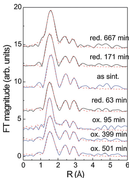
Fig. 7. Fourier transform of k^3 -weighted V EXAFS spectra of \text{Li}_{2-x}\text{VTiO}_4 sample during the process of oxidation and reduction, calculated in the k range of 4\text{--}14\text{Å}^{-1} . Experiment—solid line; EXAFS model—dashed line.
